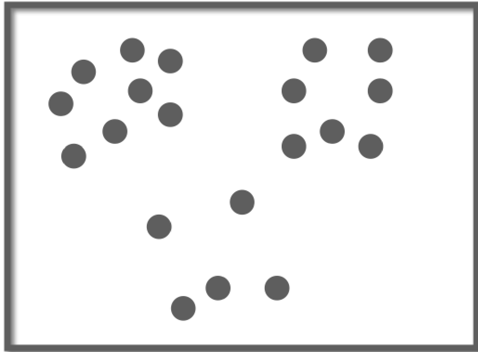
Unlabelled Data
