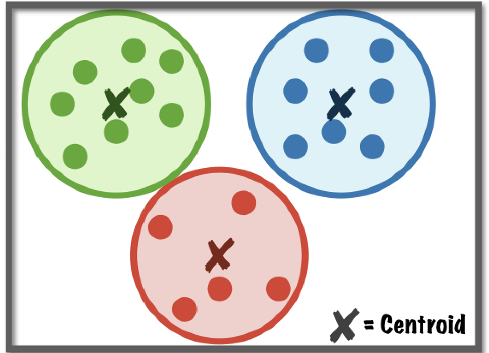
Labelled Clusters
